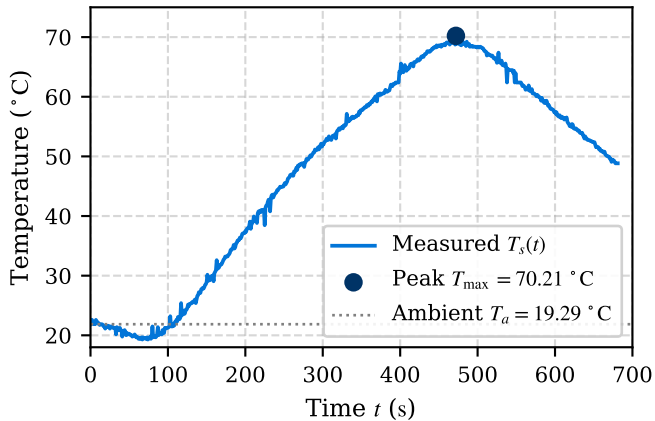
(b) Trial 2: Extended thermal cycle
