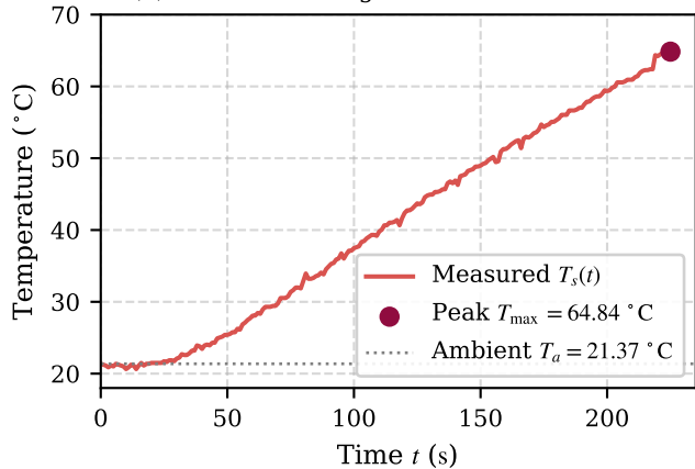
(a) Trial 1: Heating under continuous stall
